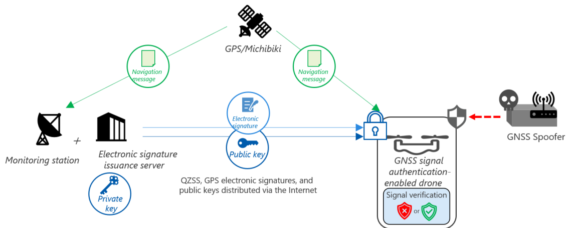
Fig. 4-9-2 System architecture
